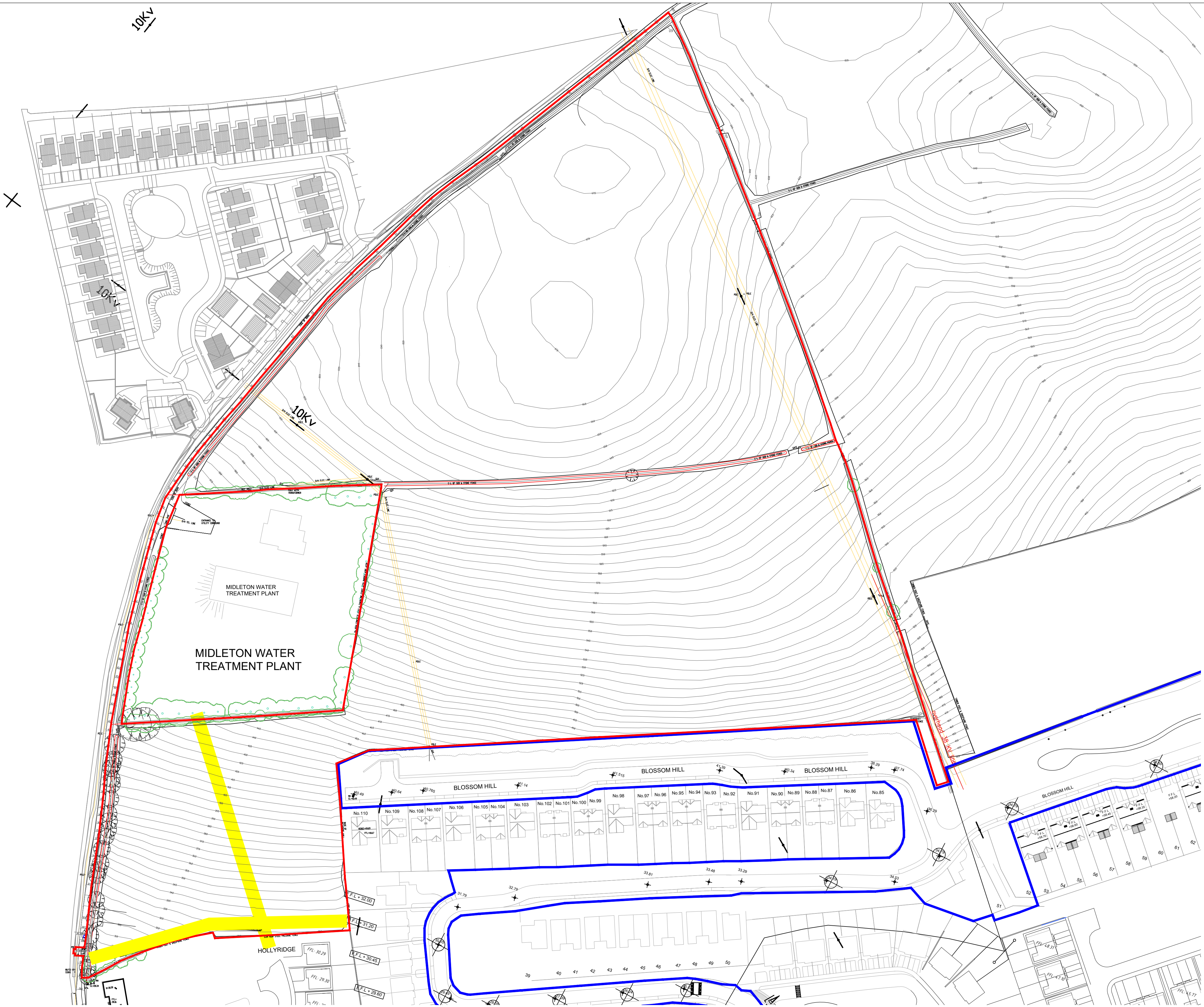
EXISTING SITE LAYOUT PLAN - TOPOGRAPHICAL SURVEY Scale 1 : 1000
