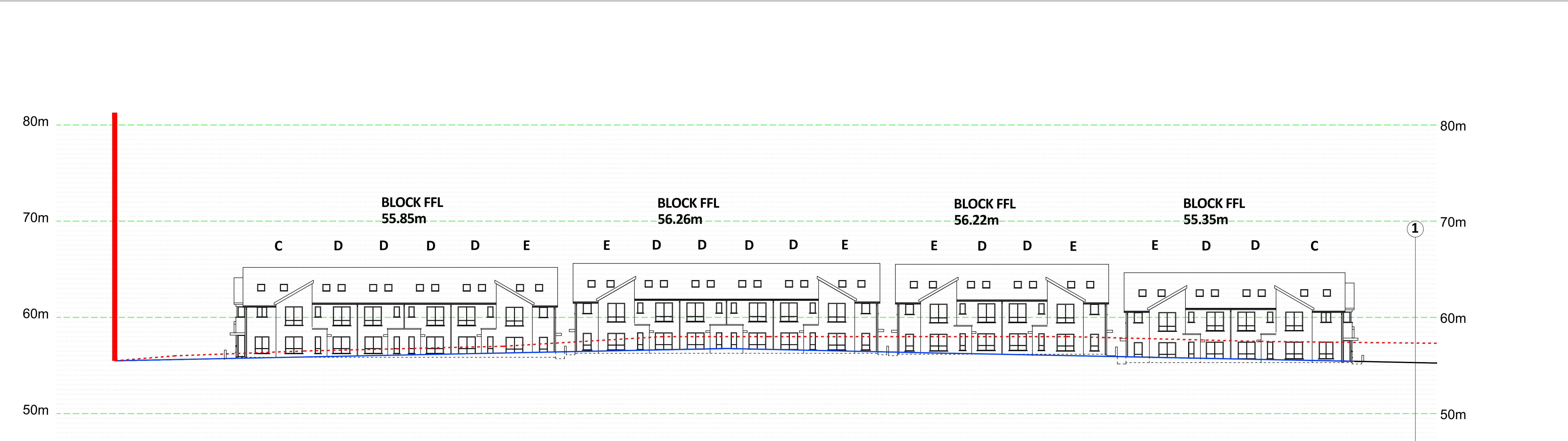
STREET ELEVATION D (part 1)
