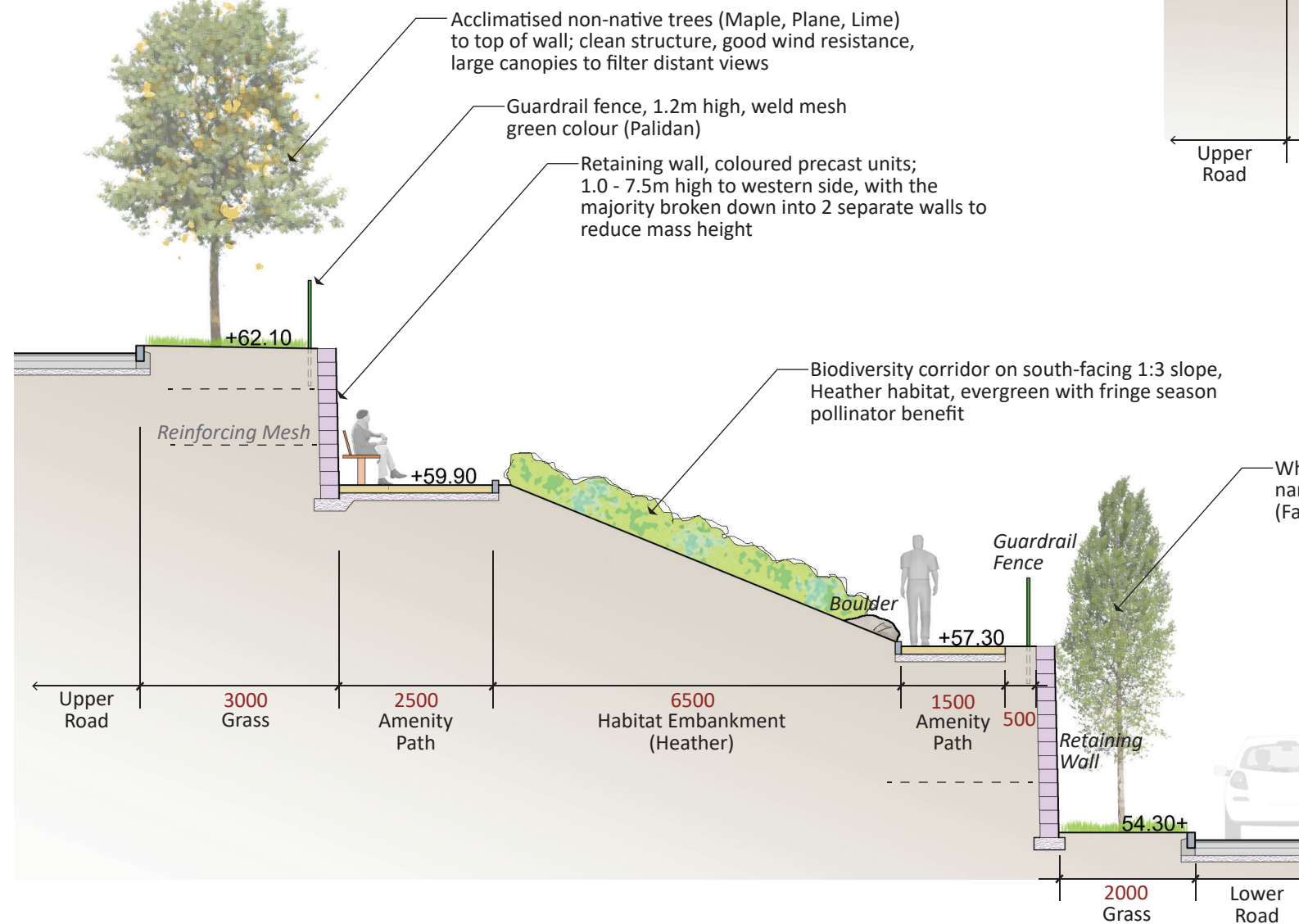
SECTION L4 - THROUGH LINEAR AMENITY, WESTERN SIDE
