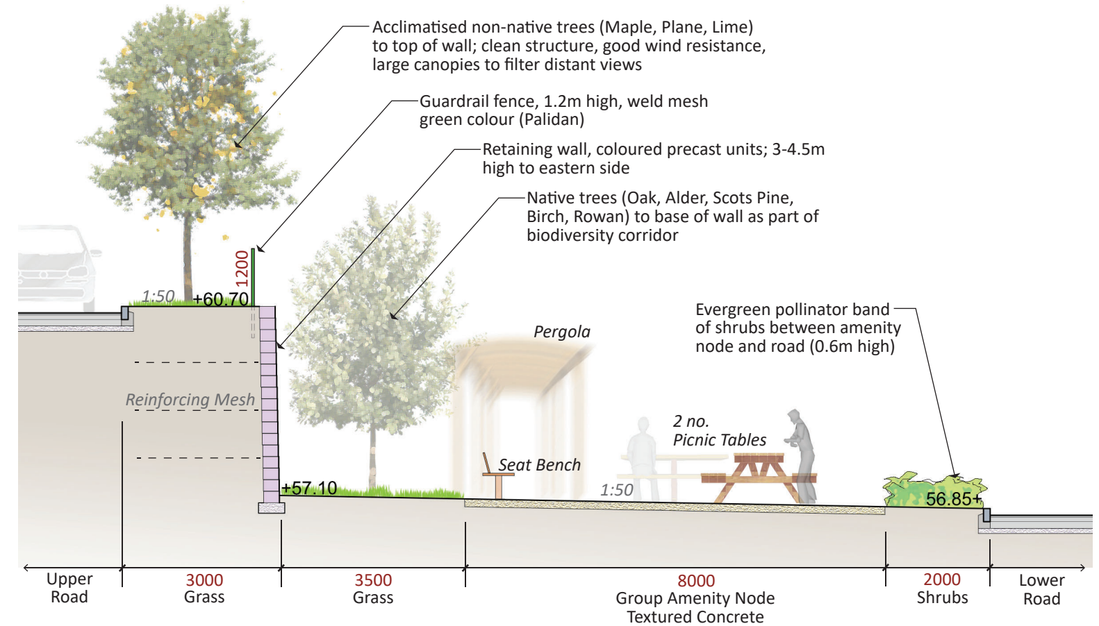
SECTION L5 - THROUGH LINEAR AMENITY, EASTERN SIDE
