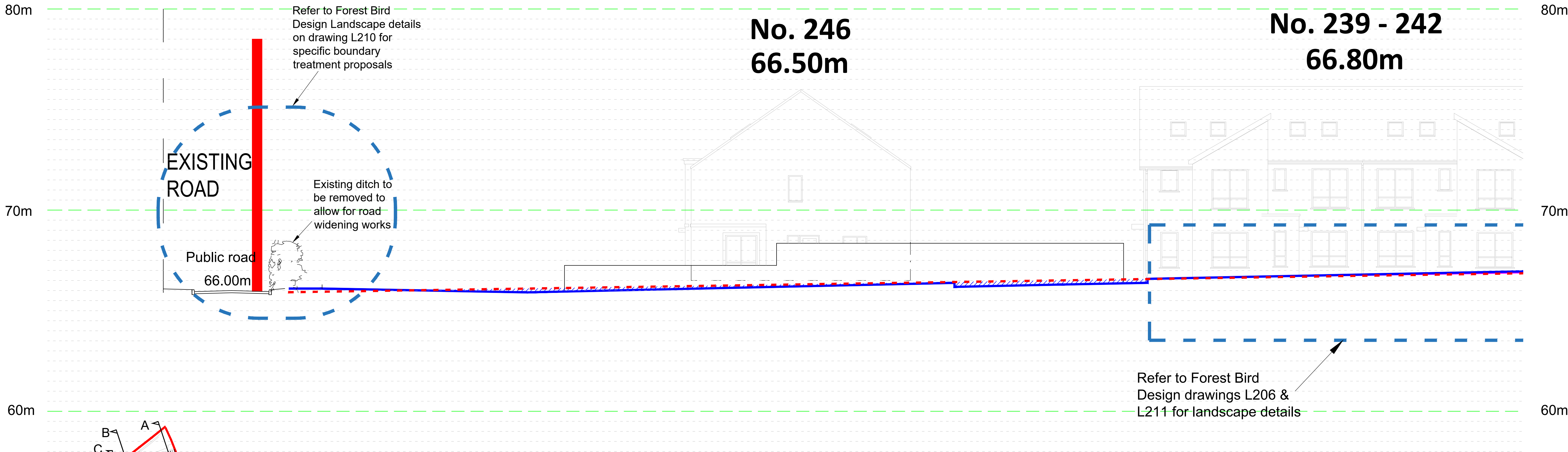
SITE SECTION G-G (part 1)
